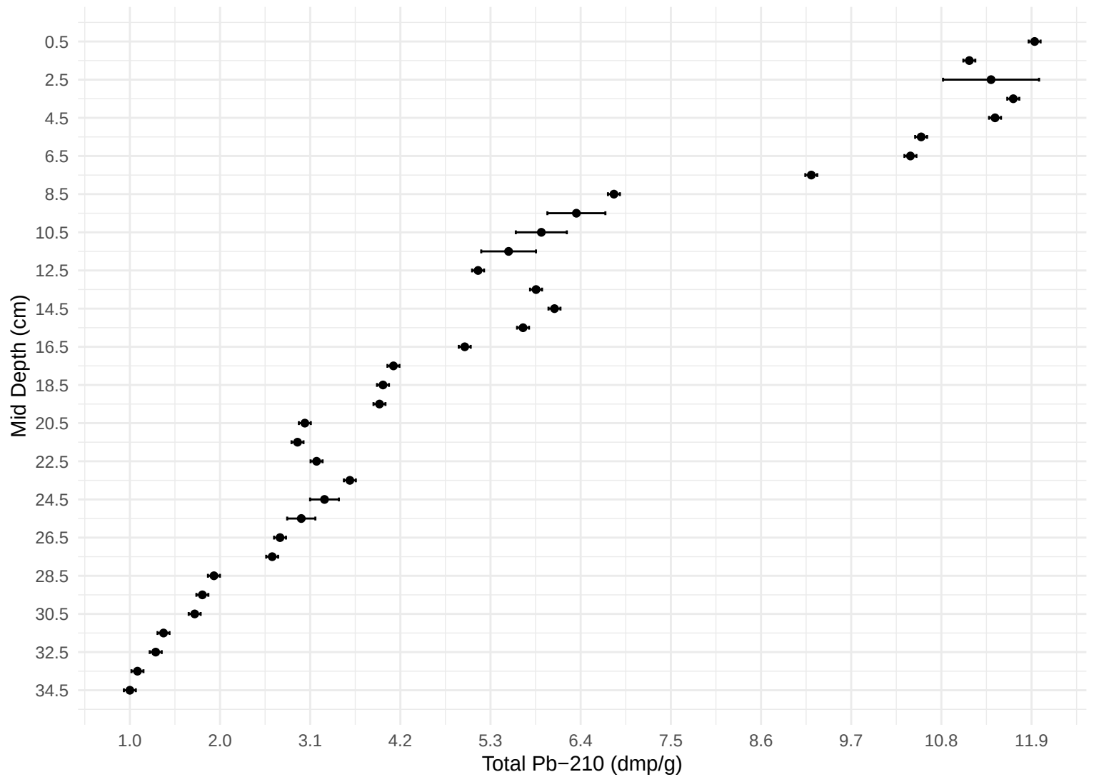
Total Pb-210 vs Depth
